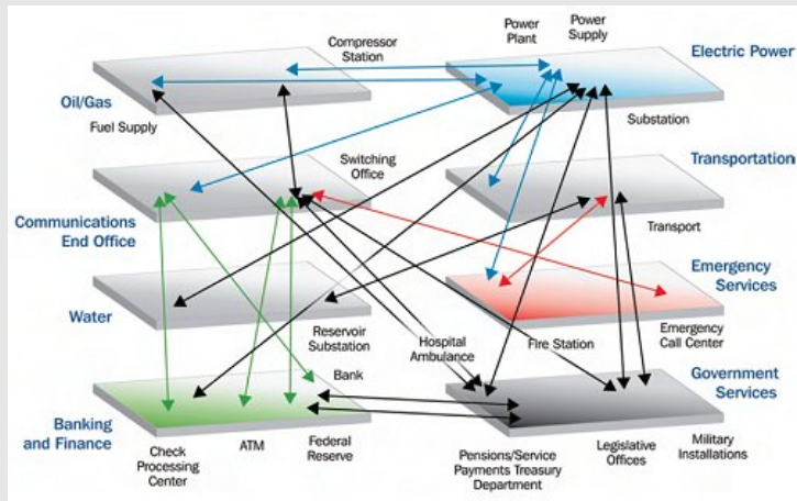
Above: A web of interdependencies makes the modern economy especially sensitive to solar storms. Source: Dept. of Homeland Security. [ Larger image ]
